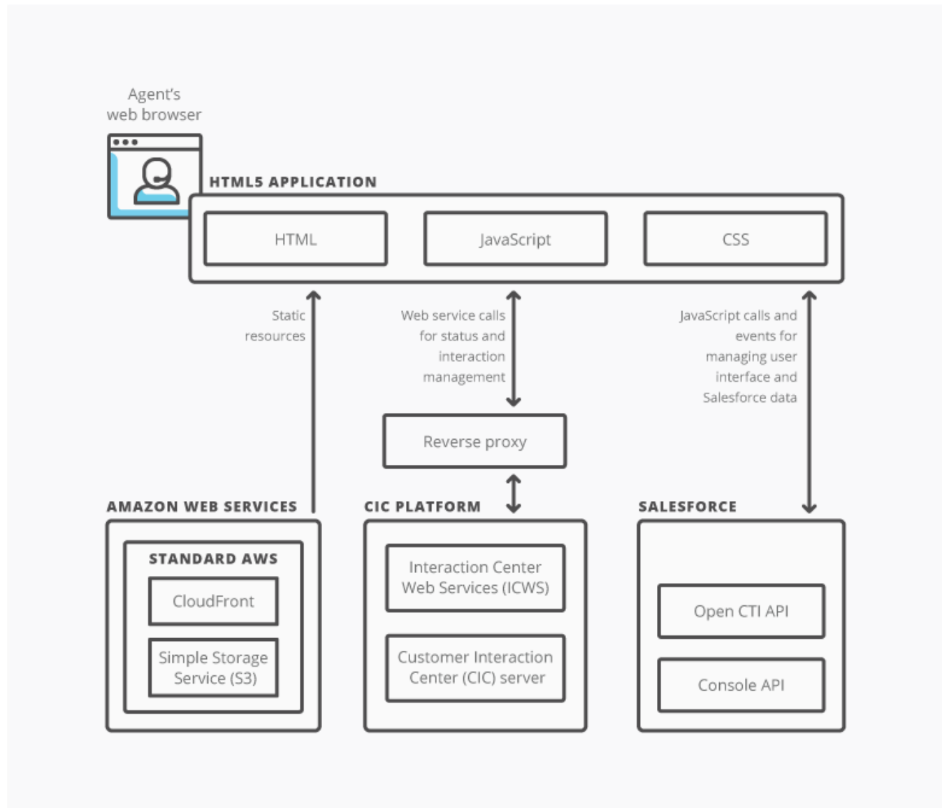
CIC for Salesforce architecture
