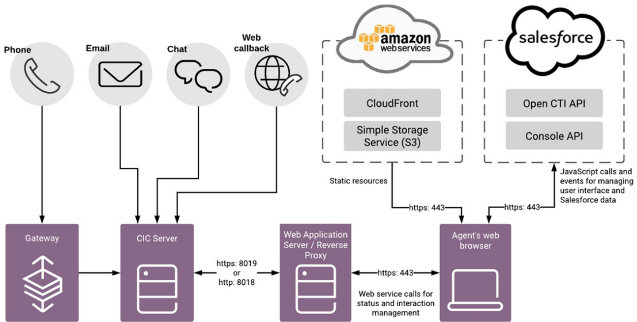
PureConnect for Salesforce Architecture
